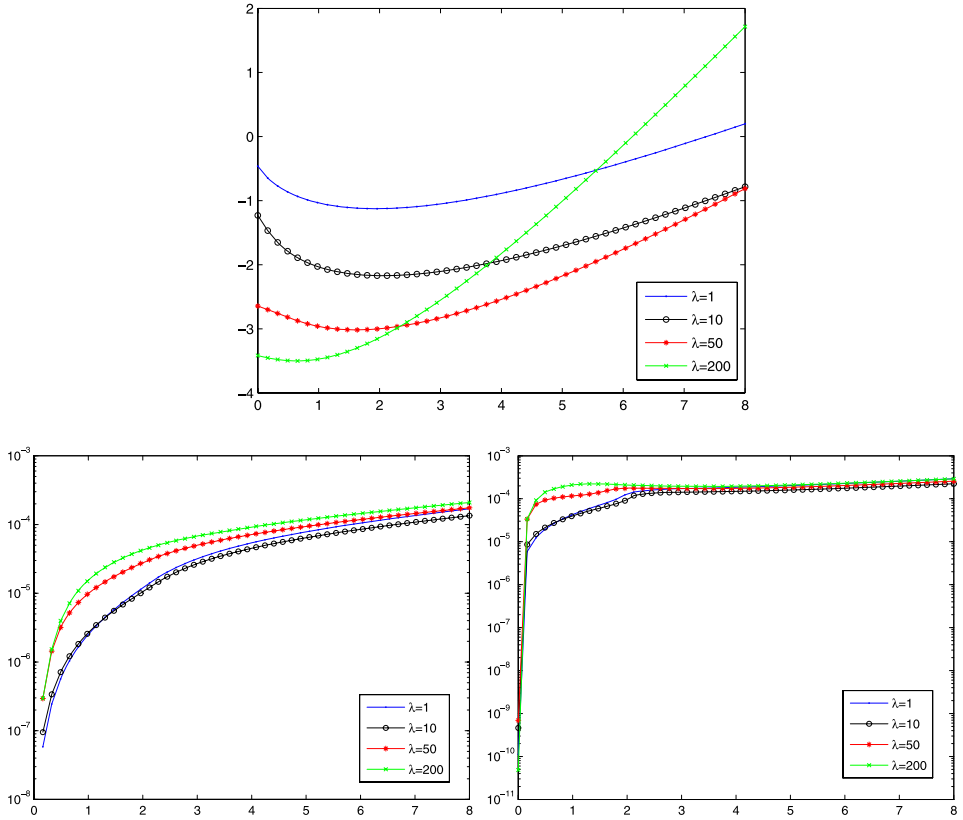
FIG. 2. In this figure we fixed the standard deviation to \sigma = 0.25 and the rate parameter to \nu = 0.125 . The first row gives the barriers for the killing parameters \lambda = 1, 10, 50, 200 . The first and second panels in the second row give the relative errors for the survival function (resp., the hazard function).
