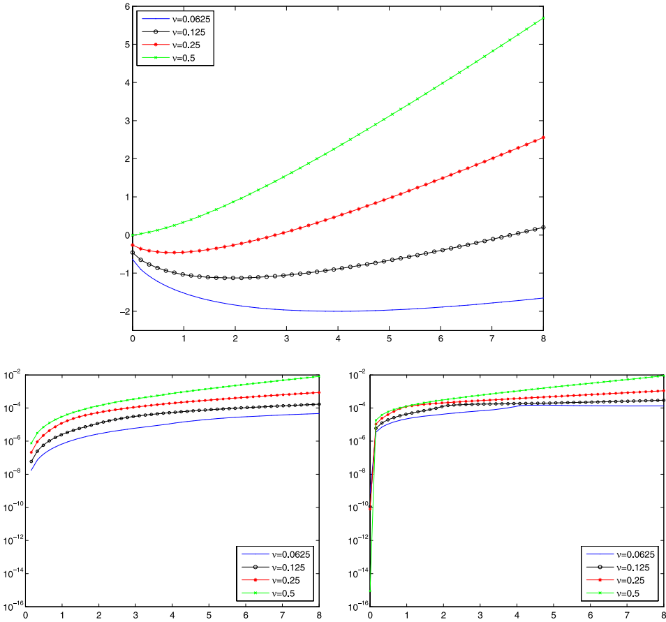
FIG. 1. This figure displays the results of the numerical experiments described in Section 6. We fix the standard deviation for the initial distribution of the credit index process Y to be \sigma = 0.25 and the killing parameter to be \lambda = 1 . The first row gives the barriers for the rate parameters \nu = 0.0625, 0.125, 0.25, 0.5 of the exponential default time distribution. The first (resp., second) panels in the second row give the relative errors between the actual survival function values G(t) [resp., the actual hazard function values -g(t)/G(t) ] and the numerically computed ones; see the text for details.
