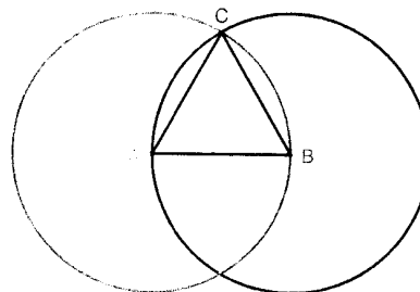
When A and B are the centers of the circles, the triangle ABC is equilateral.
