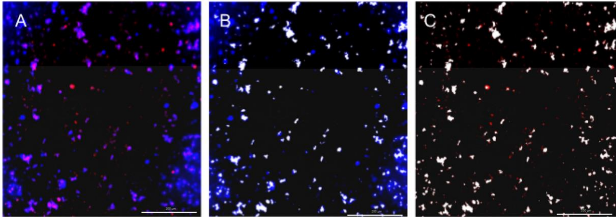
Figure 6. Fluorescence images of nanoparticles conjugated with PSTAT3 and anti-rVEGF. Red signifies the presence of anti-rVEGF, and blue signifies the presence of PSTAT3. White signifies the area where the two signals overlap. (A) Fluorescence signals of both antibodies. (B) PSTAT3 signal with the area of overlap shown. (C) anti-rVEGF signal with the area of overlap shown.
